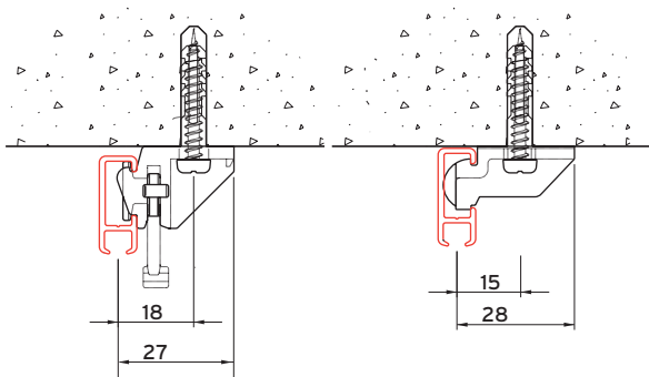
ceiling mounted with 7450 ceiling mounted with 2250
