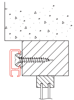
secret fixing with button clip 2254
