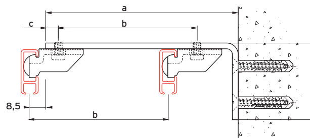
wall mounted with extension bracket 2015-10
