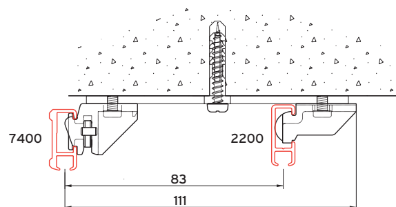
ceiling mounted with double bracket 2216 and 7450 or 2250
