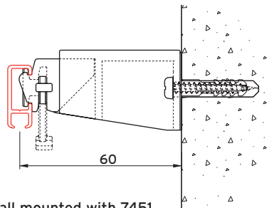
wall mounted with 7451
