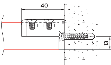
Wall fixing 5100 with wall support 5150
