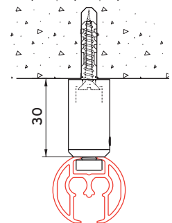
Ceiling fixing 5100 with mini-suspension hanger 4254
