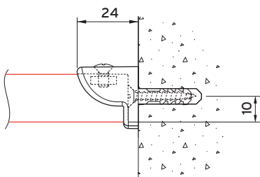
Wall fixing 4200 with wall support 4249
