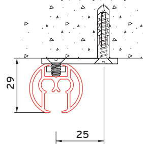
Ceiling fixing 5100 with bracket 5135
