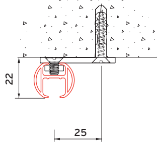
Ceiling fixing 4200 with bracket 5135
