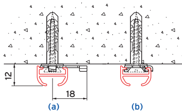
Ceiling fixing with fixing clamp 2650 (including washer), before (a) and after (b) tightening the fixing clamp
