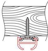
Ceiling fixing with clamp 2650 including washer and screw 2614
