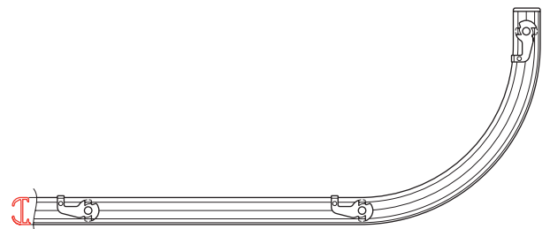
When installing a bent profile, position a fixing clamp directly before and after each curve
